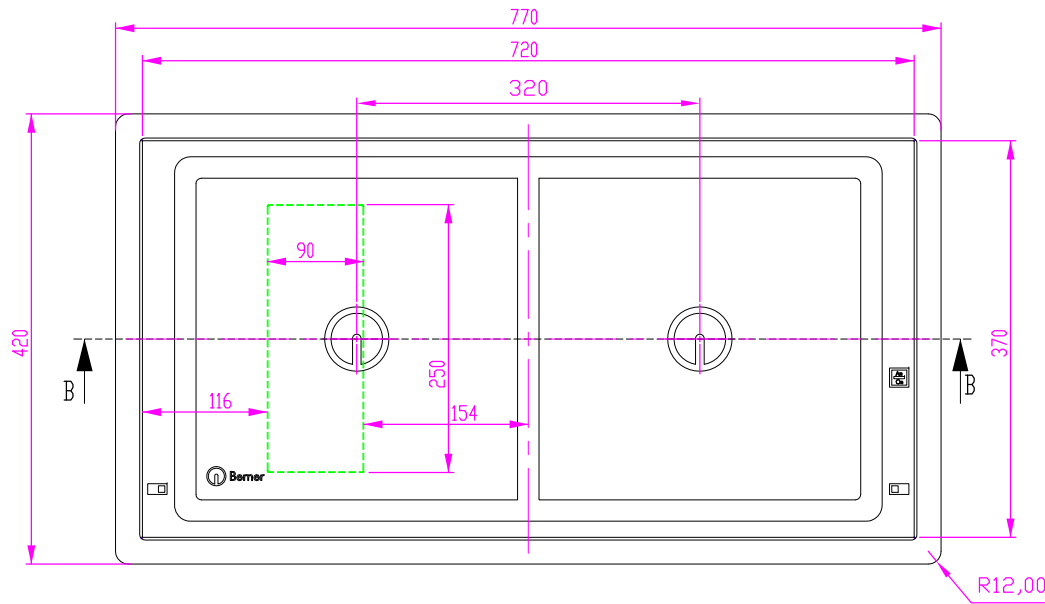
Ausschnitt in Abdeckung 750 x 400 cut out at cover panel
