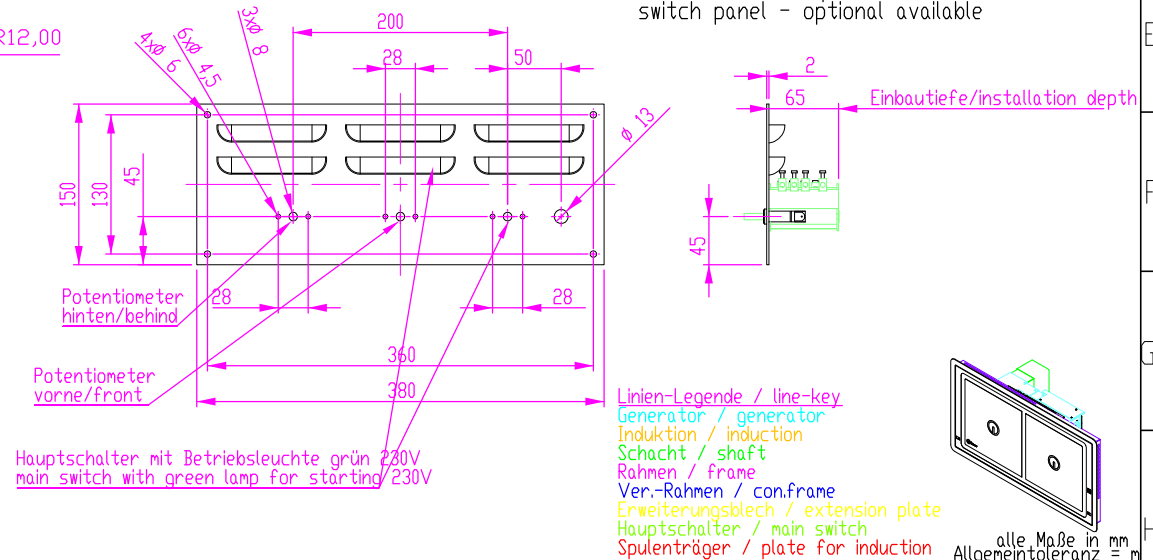
Schalterblende (optional lieferbar) switch panel - optional available
