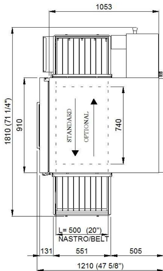
TOP VIEW
